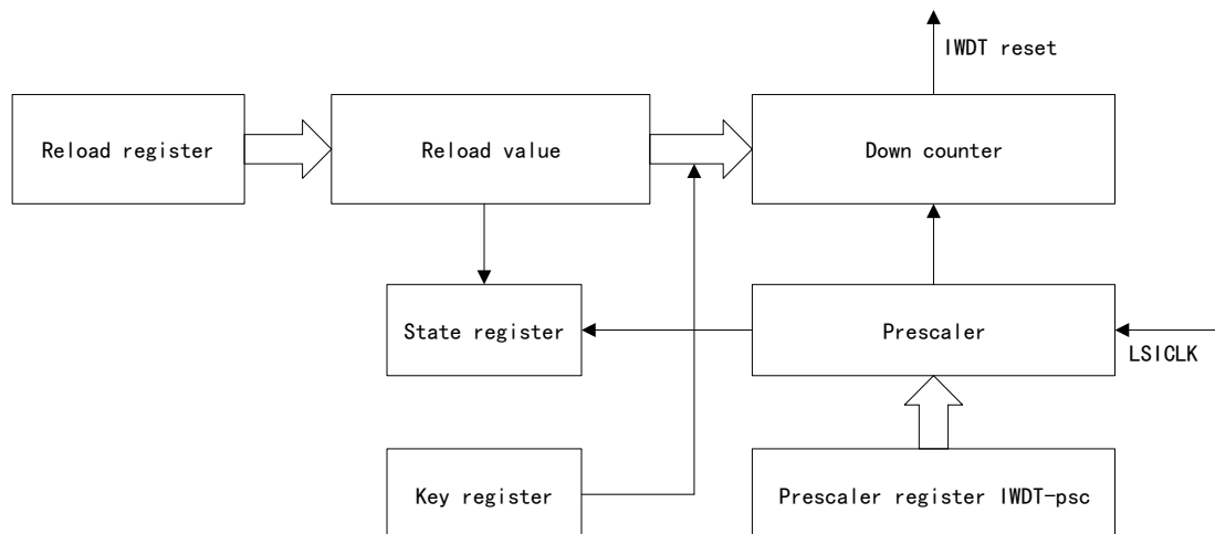
Figure 79 Independent Watchdog Structure Block Diagram
